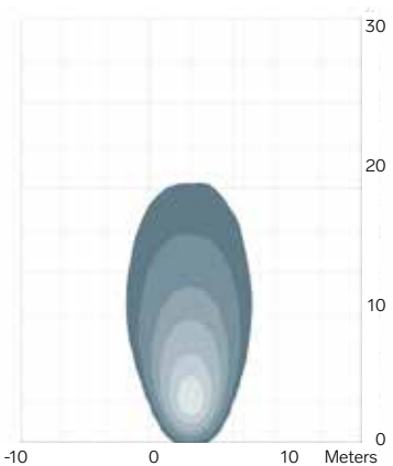
1313 AC / 3700 lm Wide 45°+ 3.0 m / -15° Symmetric
