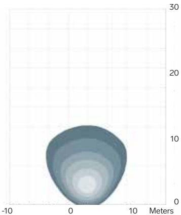
1313 AC / 3700 lm Wide 45°+ 3.0 m / -15° Asymmetric
