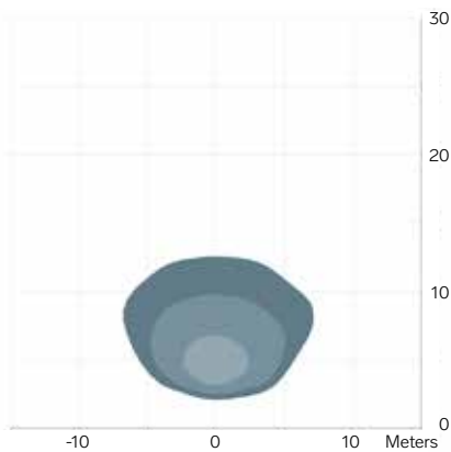
1010 Flush / 700 lm Wide 45°+ 3.0 m / -15° Symmetric
