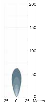
1010 Flush / 700 lm High 1.0 m / 0° Symmetric
