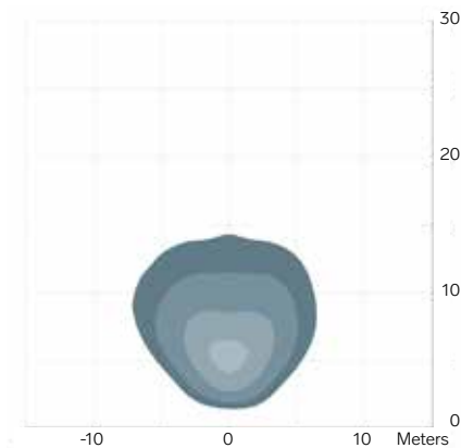
1010 Flush / 700 lm Wide 45°+ 3.0 m / -15° Asymmetric
